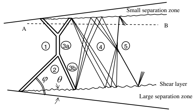
Fig. 13 Simplified schematic of the shock and flow structure.
