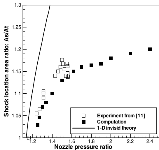
Fig. 8 Shock location versus nozzle pressure ratio.
